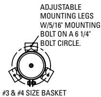
#3 & #4 SIZE BASKET
