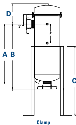
Clamp
