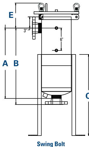
Swing Bolt
