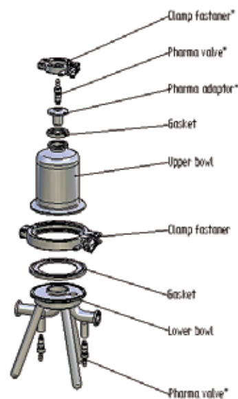
Pharma valves on PF-EG 0003 to 0075 only
